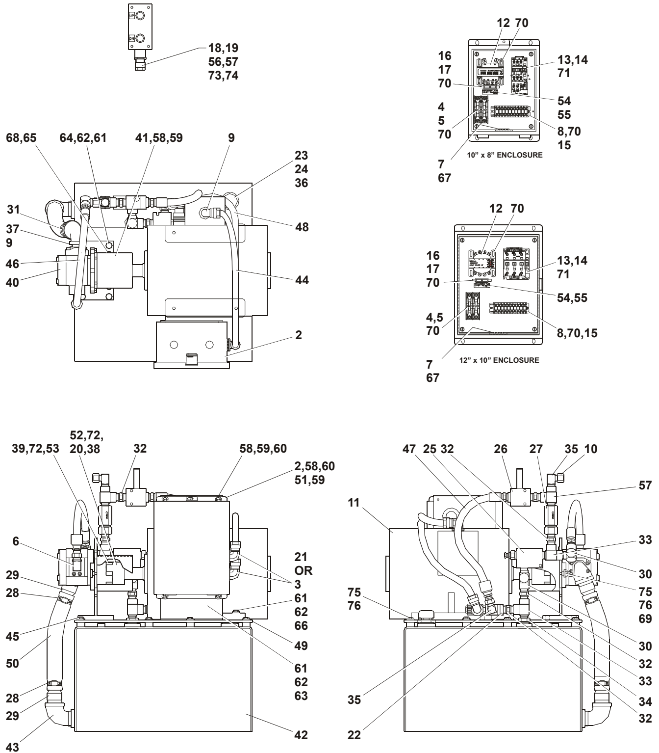
Figure 53 : Power Pack - 10 Horse Power
