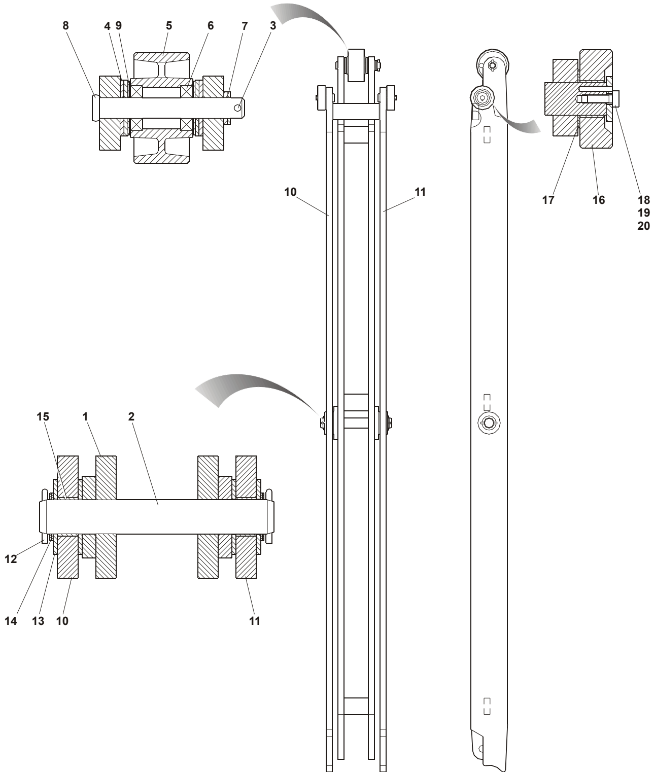
Figure 59 : Leg Assembly - 4, & 5,000 lb. Cap. - 72x120" Deck Length
