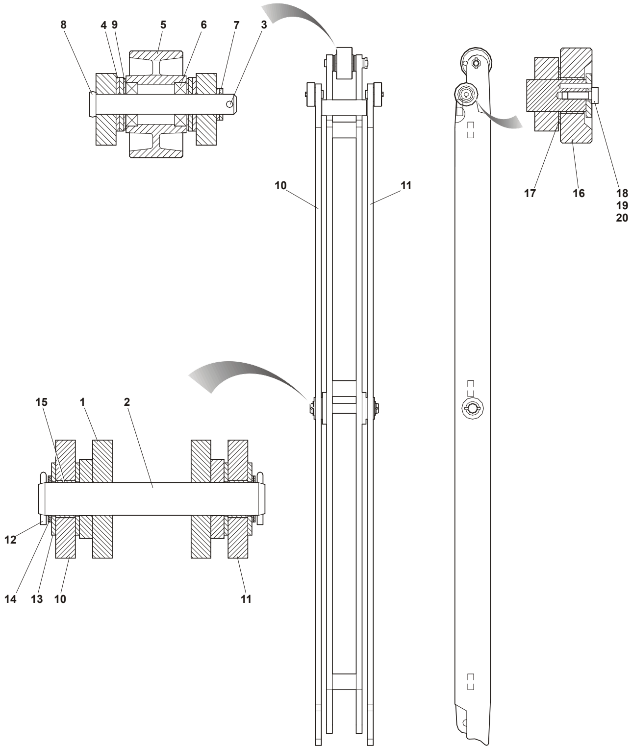
Figure 63 : Leg Assembly - 4, & 5,000 lb. Cap. - 84x96" Deck Length
